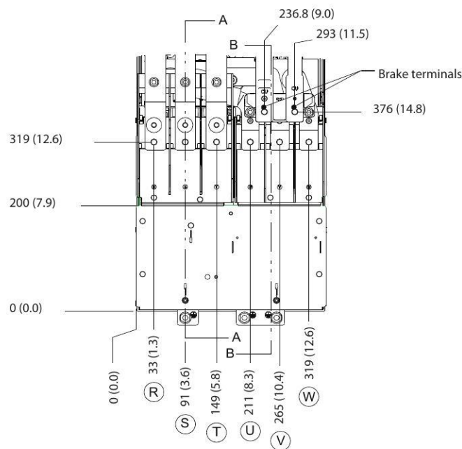
Illustration 7.3 Drive Module Terminal Dimensions (Front View)
