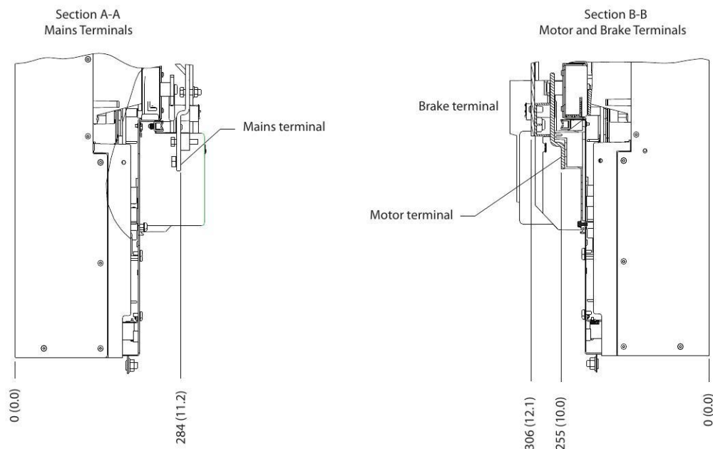
Illustration 7.4 Drive Module Terminal Dimensions (Side Views)
