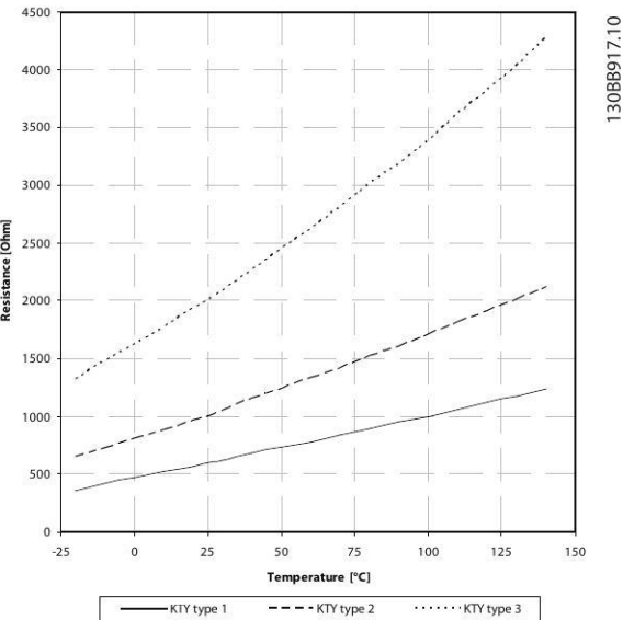
Illustration 5.6 KTY Type Selection
