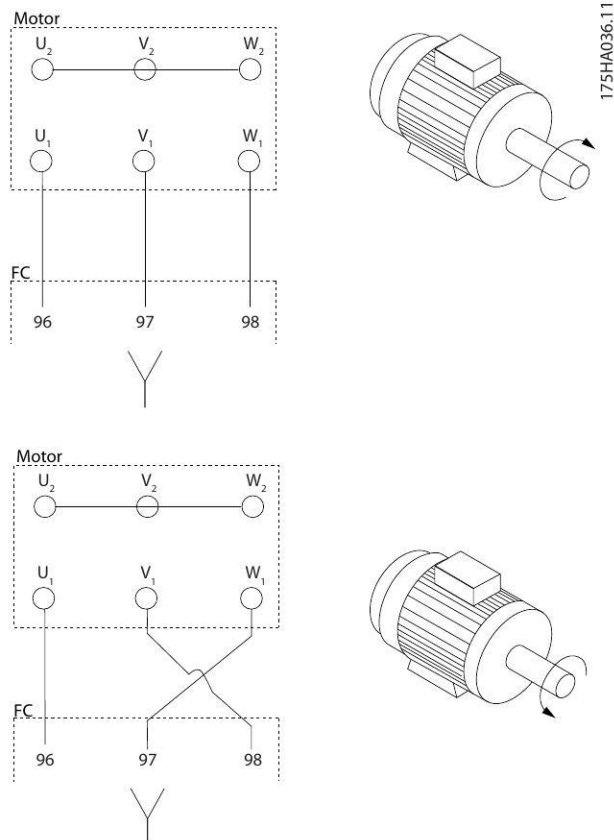
Illustration 5.7 Changing Motor Rotation
