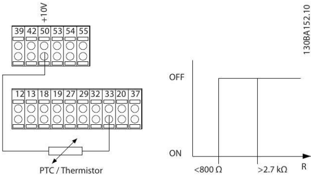
Illustration 5.3 PTC Thermistor Connection - Digital Input with 10 V Supply
