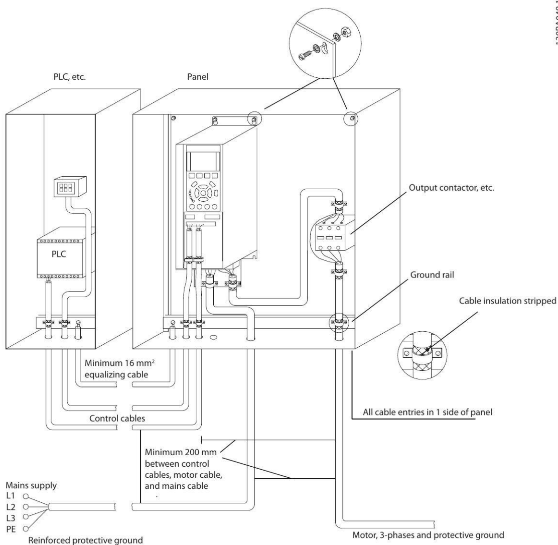
Illustration 5.13 EMC-correct Electrical Installation of a Frequency Converter in Cabinet
