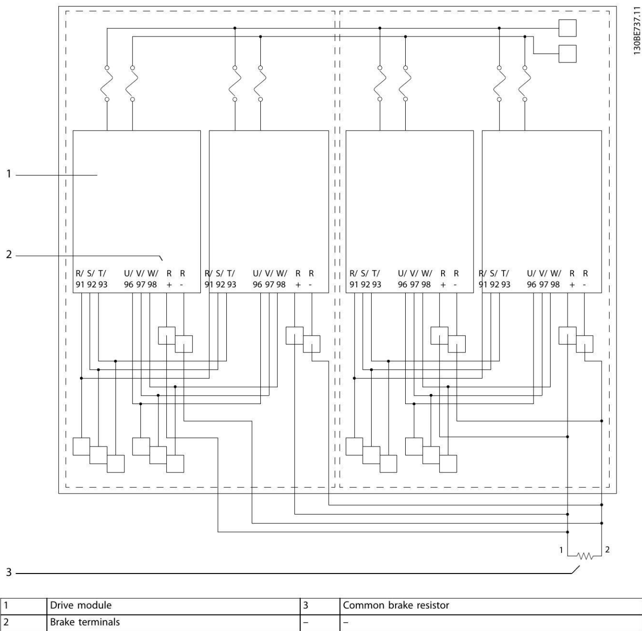
Illustration 8.4 Connection of Common Brake Resistor
