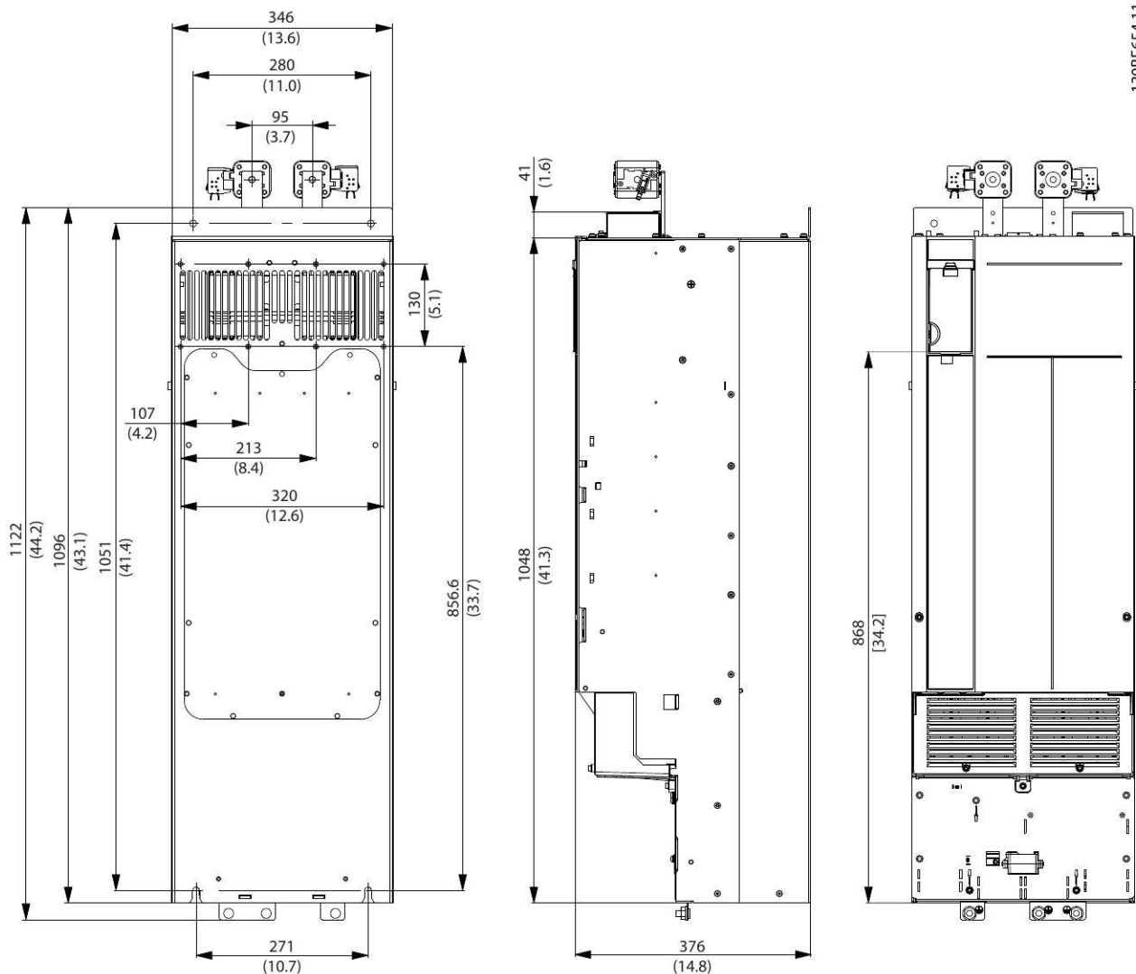
Illustration 7.2 VLT® Parallel Drive Modules Installation Dimensions
