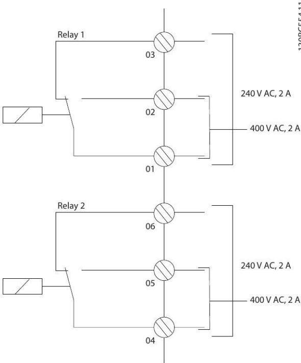
Illustration 5.12 Extra Relay Outputs
