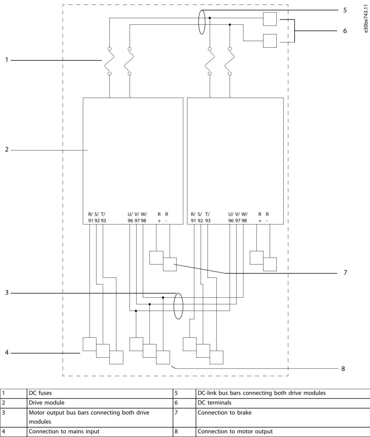
Illustration 8.10 Connections in a 12-Pulse 2-Drive Module System
