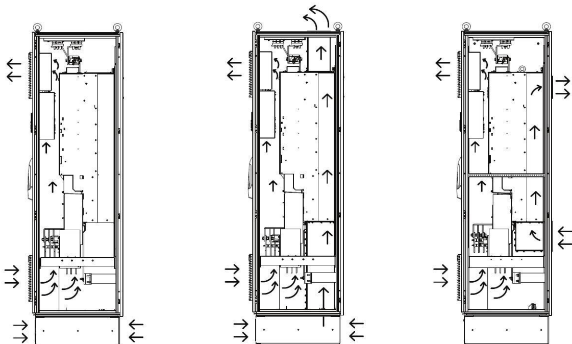
Illustration 4.4 Airflow, Standard Unit (Left), Bottom/Top Cooling Kit (Middle), and Back/Back Cooling Kit (Right)
