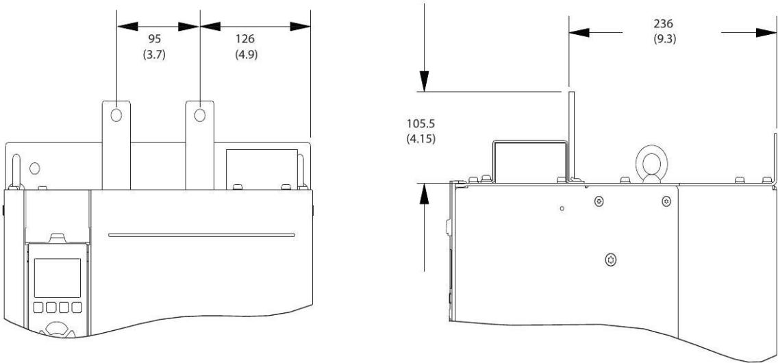
Illustration 7.5 DC Bus Dimensions (Front and Side Views)
