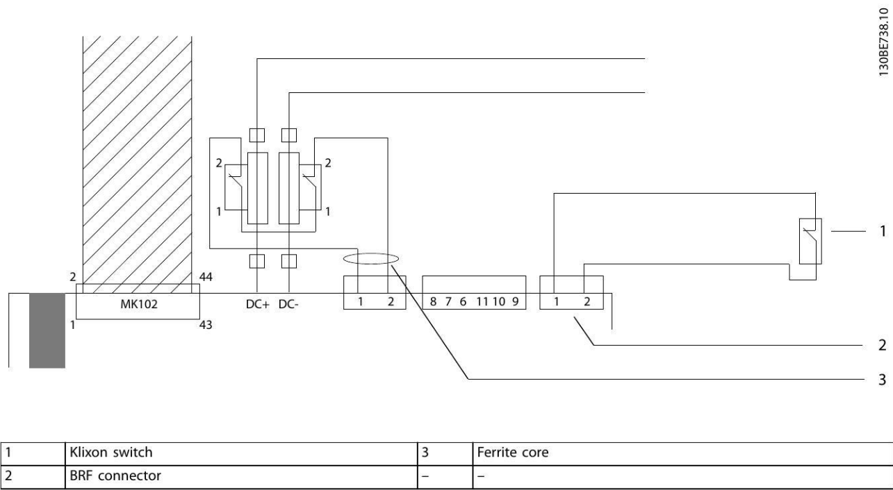
Illustration 8.5 Klixon Switch Connection
