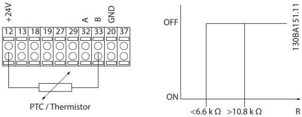
Illustration 5.5 PTC Thermistor Connection - Digital Input with 24 V Supply
