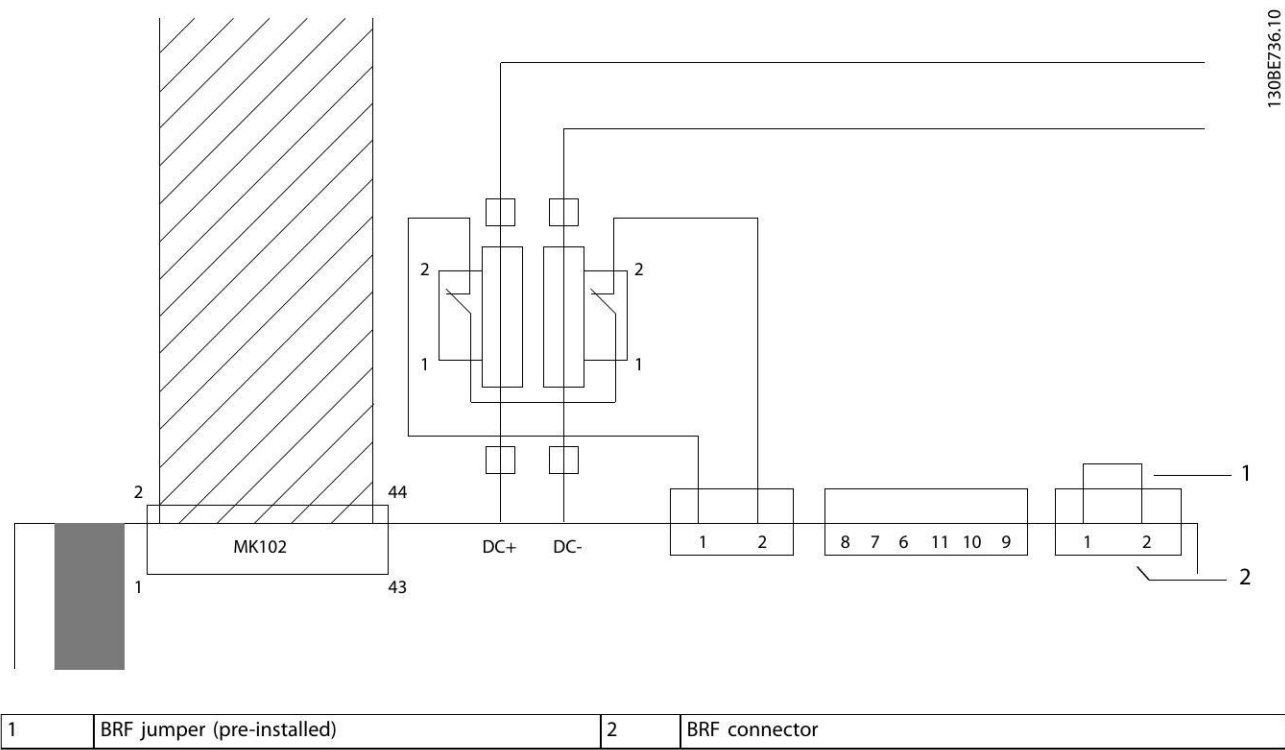
Illustration 8.3 BRF Jumper Connection
