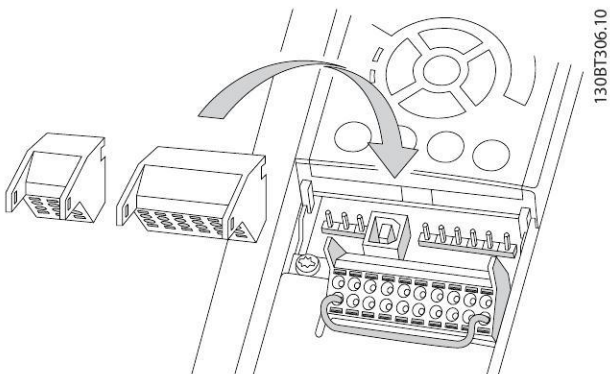
Illustration 5.10 Removal of Control Terminals
