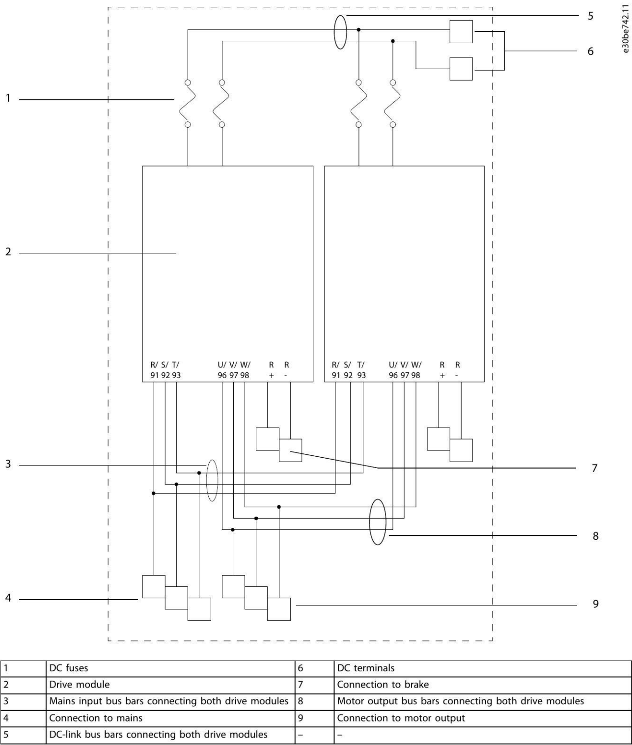
Illustration 8.9 Connections in a 6-Pulse 2-Drive Module System
